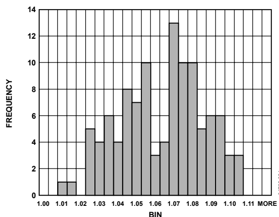
Figure 24. I_{BD} Histogram @ V_{DD} = 5V
