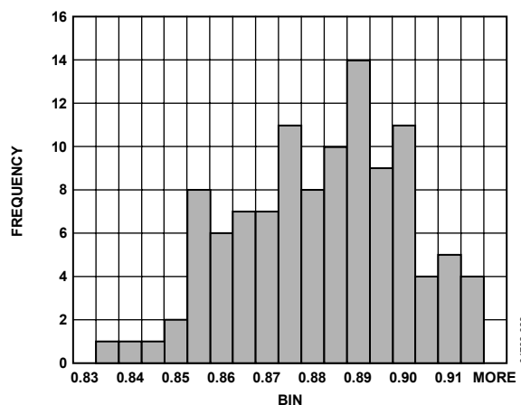
Figure 23. I_{BD} Histogram @ V_{DD} = 3V
