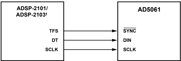
Figure 40. AD5061-to-ADSP-2101/ADSP-2103 Interface
