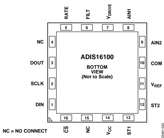
Figure 4. Pin Configuration
