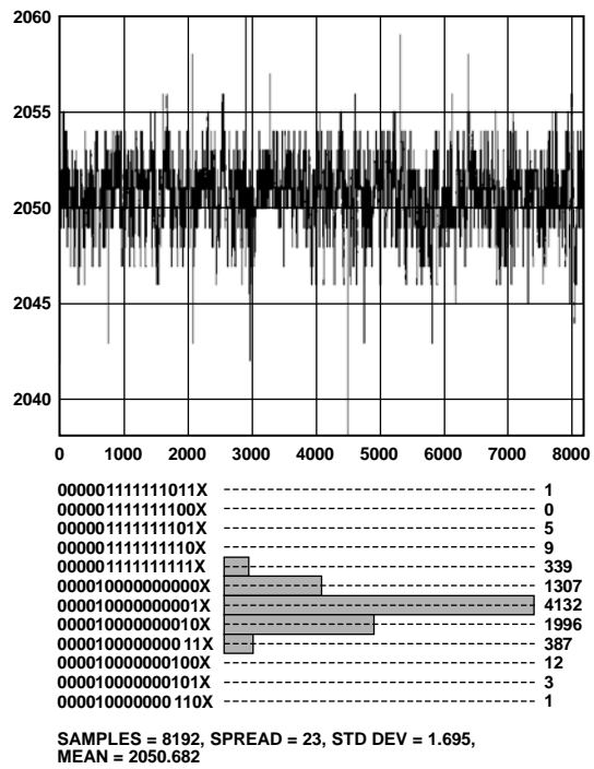
Figure 18. Noise Histogram
