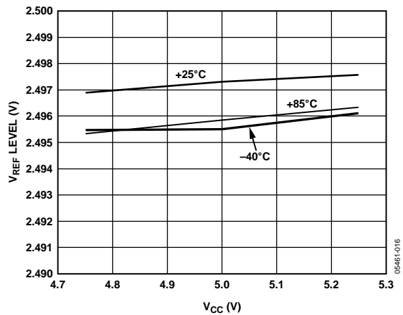
Figure 17. V_{REF} vs. Supply Voltage
