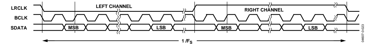
Figure 16. I 2 S Mode—16 to 24 Bits per Channel
