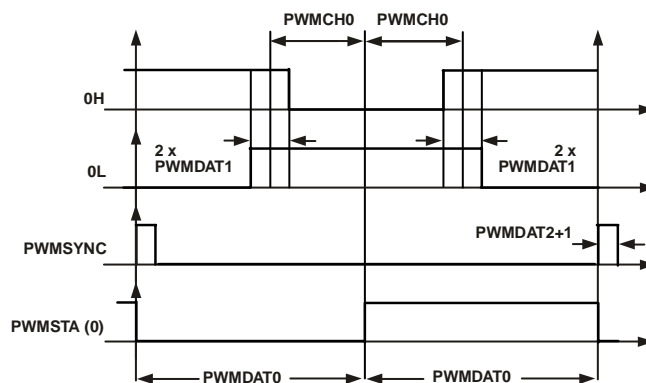
Figure 22: Typical PWM outputs of Three-Phase timing unit in single update mode
