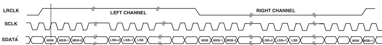
Figure 29. Left-Justified Mode
