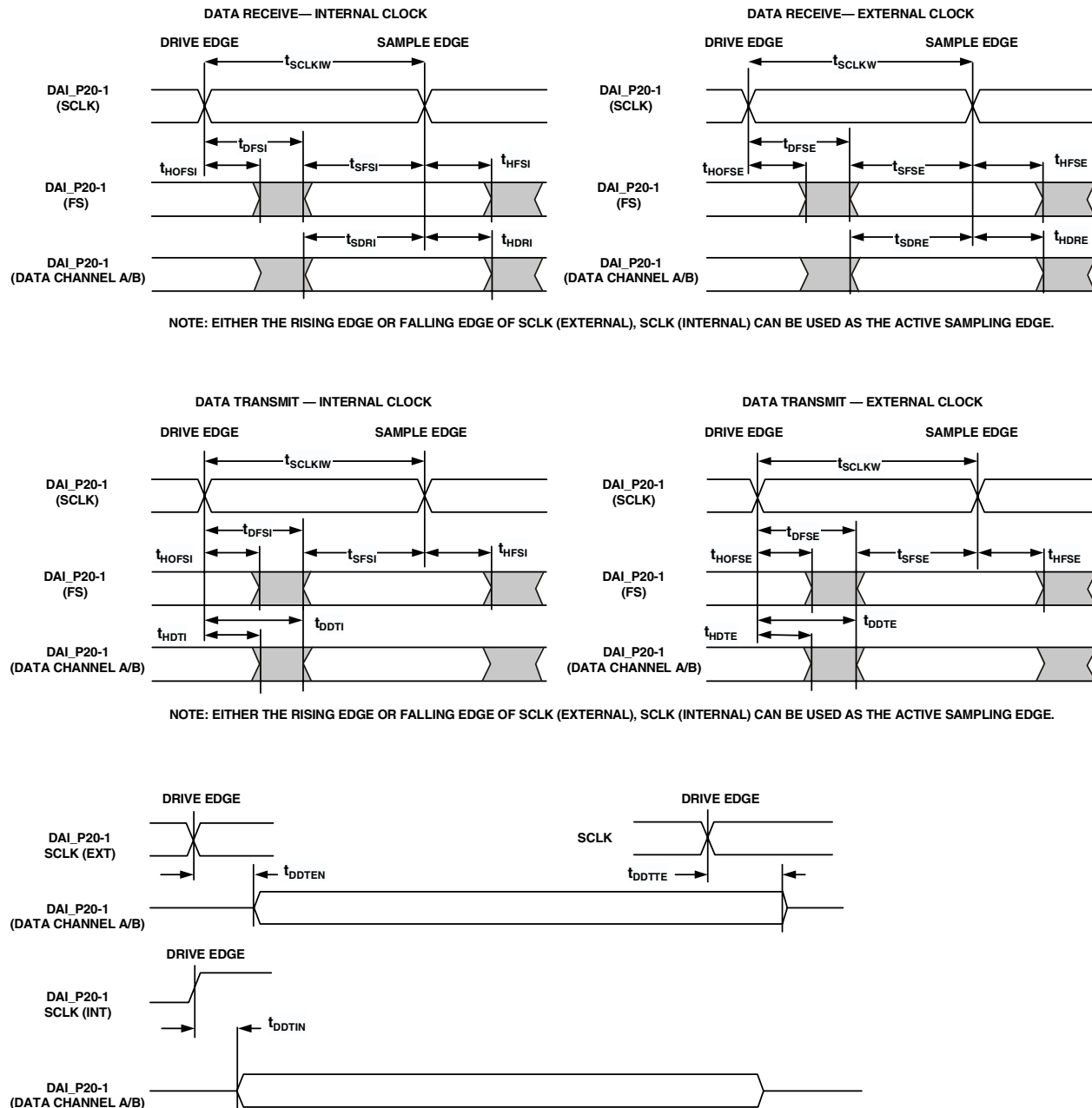
Figure 22. Serial Ports
