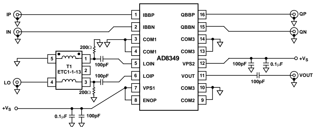
Figure 43. Basic Connections
