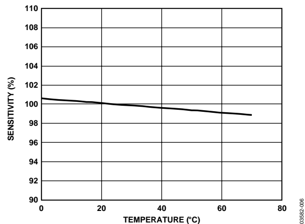
Figure 7. Normalized Sensitivity vs. Temperature
