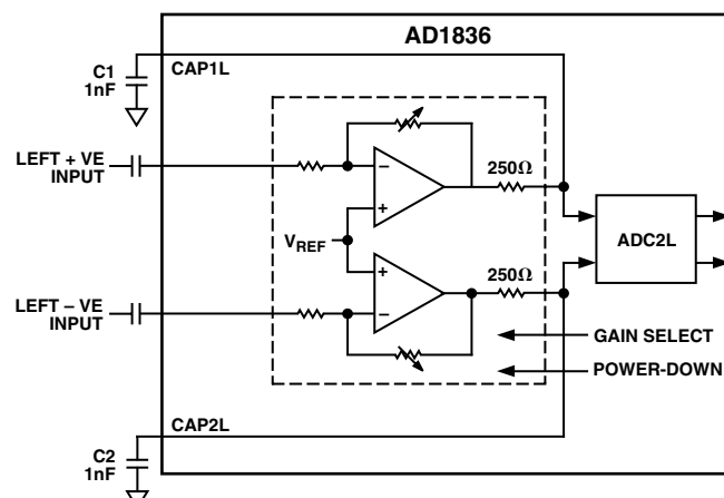
Figure 13. Differential Mode
