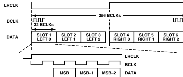
Figure 7. DAC Packed Mode 256
