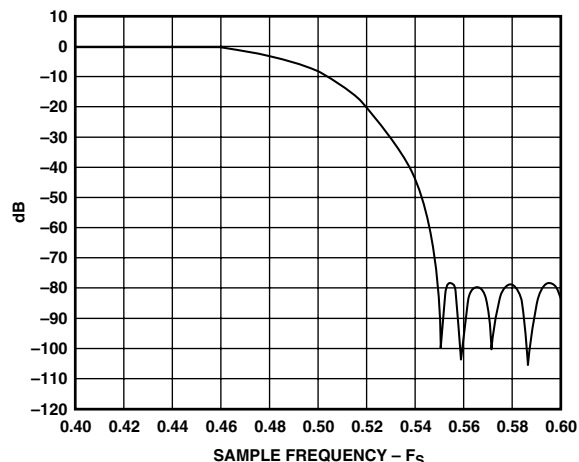
Figure 25. Analog-to-Digital Frequency Response—Transition Band (Full-Scale Line-Level Inputs, 0 dB Gain)
