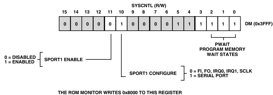
Figure 28. Configuration of Registers
