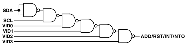
Figure 7. NAND Tree
