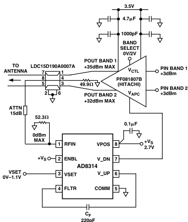
Figure 10. A Dual Mode Power Amplifier Control Circuit
