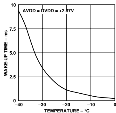
Figure 11. Wake-Up Time vs. Temperature
