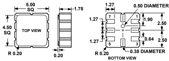
Figure 11. 8-Terminal Ceramic Leadless Chip Carrier [CLCC] (E-8) Dimensions shown in millimeters
