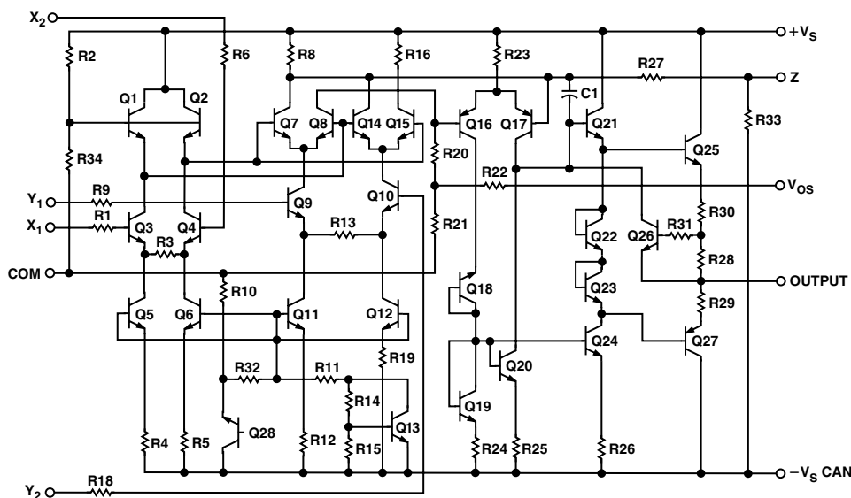
Figure 2. Schematic Diagram
