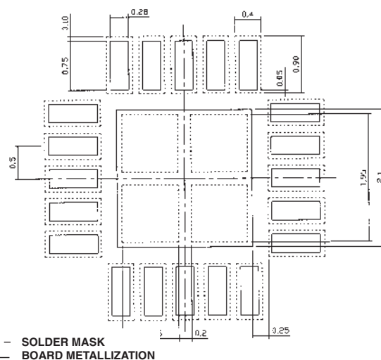
Figure 3. Suggested LFCSP 4 × 4 20-Lead Land Pattern
