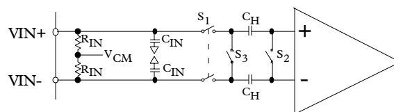
Figure #. Differential Input Architecture
