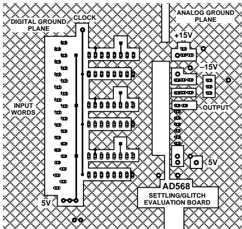
Component Side
