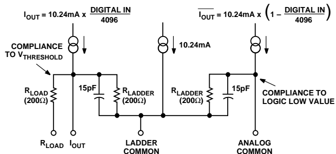
Figure 11. Equivalent Output
