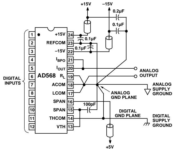
Figure 4. Bipolar Output Unbuffered \pm 0.512 V
