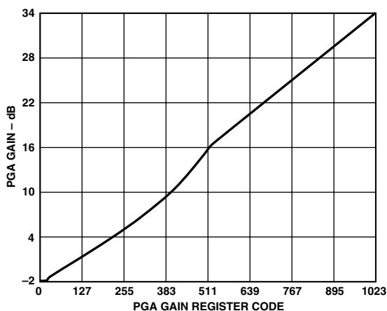
Figure 5a. PGA Gain Curve for CCD-Mode
