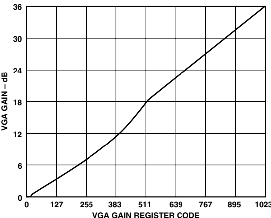
Figure 20. VGA Gain Curve (Gain from PxGA Not Included)
