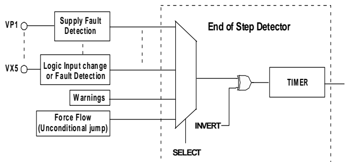
Figure 9. End-of-Step Detector
