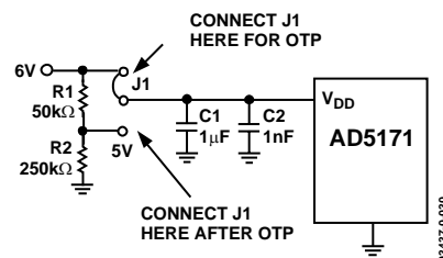
Figure 25. Power Supply Requirement
