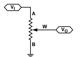
Figure 32. Potentiometer Mode Configuration
