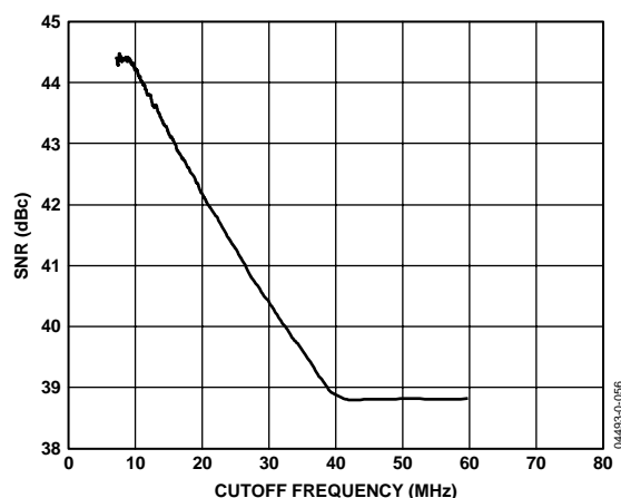
Figure 19. SNR vs. Filter Cutoff Frequency (50 MSPS; f_{\text{IN}} = 5 MHz; AIN = -1 dB; RxPGA = 48 dB)
