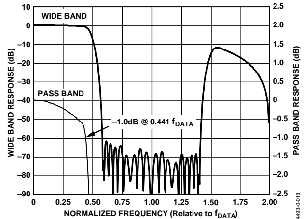
Figure 60. Frequency Response of 2\times Interpolation Filter (Normalized to f_{DATA} )
