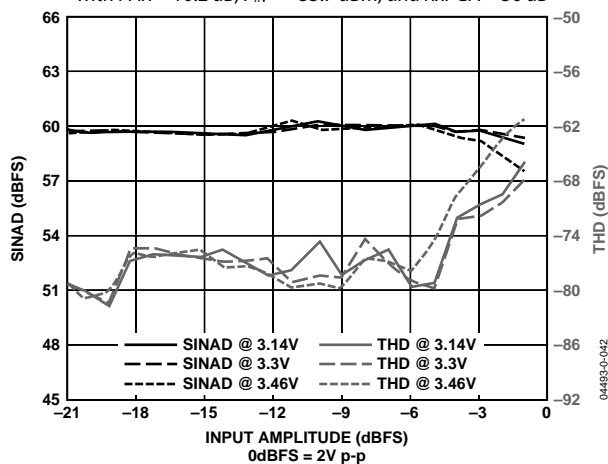
Figure 5. SINAD and THD vs. Input Amplitude and Supply f_{\text{IN}} = 8 MHz, LPF f_{-3\text{ dB}} = 26 MHz; Rx PGA = 0 dB)
