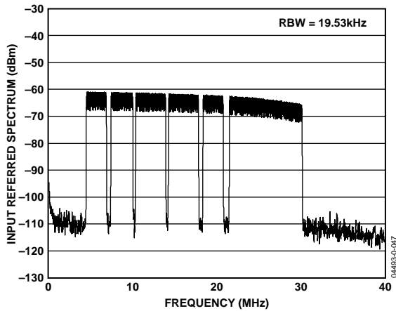
Figure 10. Spectral Plot with 4k FFT of 111-Carrier DMT Signal with \text{PAR} = 11 dB, P_{\text{IN}} = -33.7 dBm, LPF's f_{-3\text{dB}} = 32 MHz, and RxPGA = 36 dB
