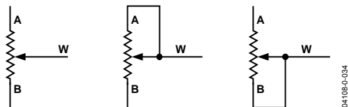
Figure 33. Rheostat Mode Configuration
