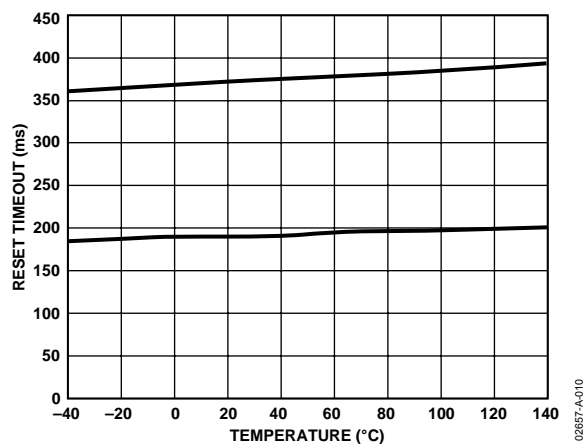
Figure 10. Power-up Reset Timeout vs. Temperature
