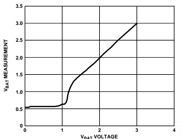
Figure 15. V_{BAT} Measurement vs. Voltage
