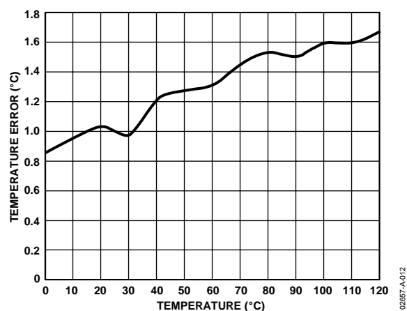
Figure 12. Local Sensor Temperature Error
