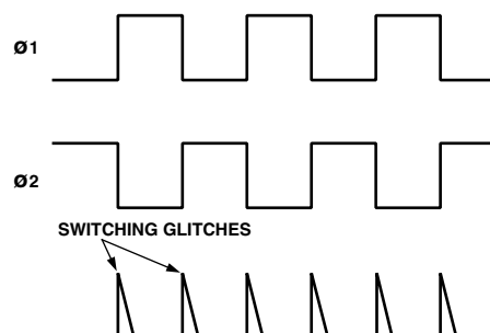
Figure 10. Switching Glitches
