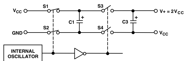
Figure 9. Charge Pump Voltage Doubler
