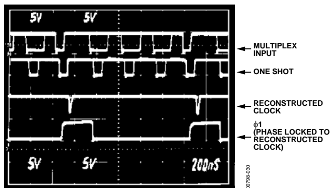
Figure 29. Demultiplexer Waveforms
