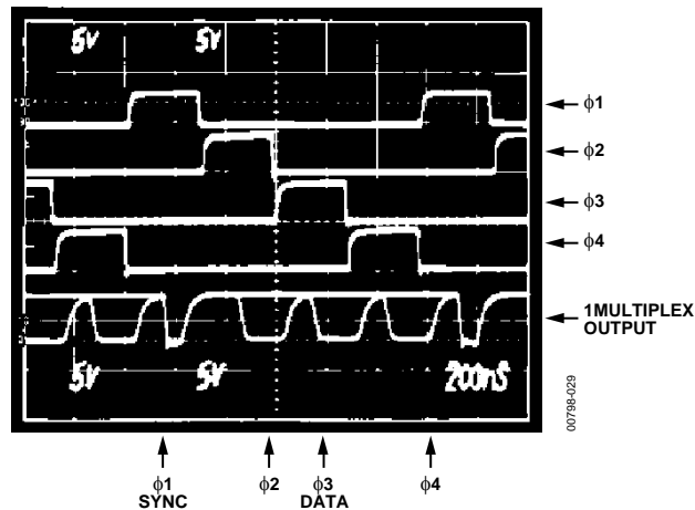
Figure 28. Multiplexer Waveforms
