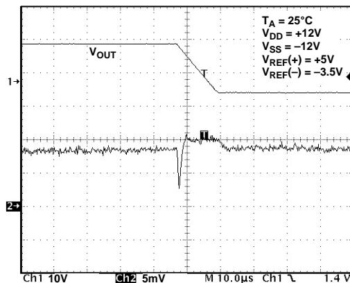
Figure 17. DAC-to-DAC Crosstalk
