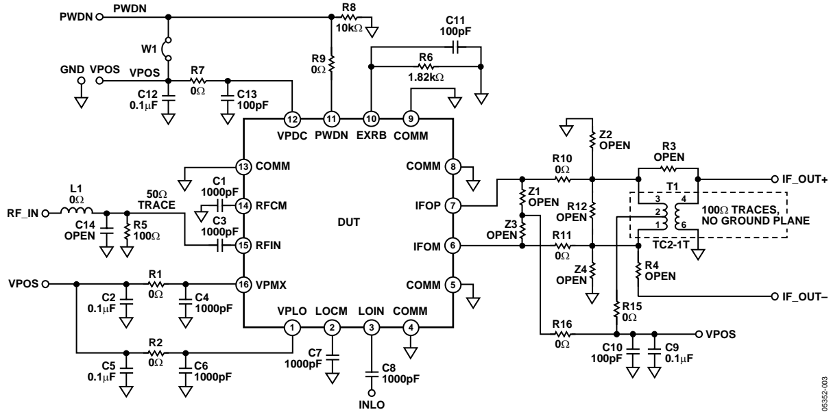
Figure 53. Evaluation Board
