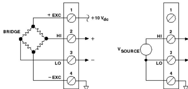
Figure 3 3B16 Input Field Connections
