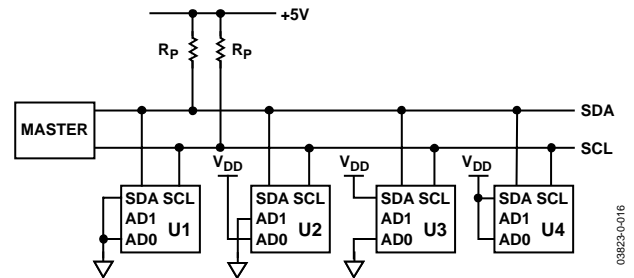
Figure 37. Multiple AD5251/AD5252s on a Single Bus
