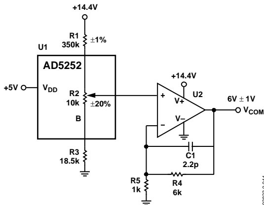
Figure 44. Apply 5 V Digital Potentiometer AD5252 in a 6 V \pm 1 V Application.
