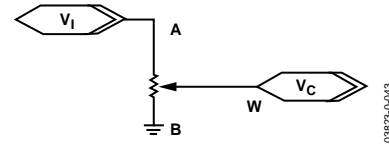
Figure 43. Potentiometer Mode Configuration
