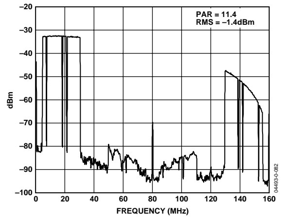
Figure 37. Wideband Spectral Plot of 111-Carrier OFDM Test Vector ( f_{DATA} = 80\text{ MSPS} , 2× Interpolation)
