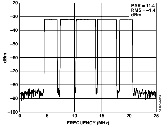
Figure 33. Spectral Plot of 84-Carrier OFDM Test Vector ( f_{DATA} = 50\text{ MSPS} , 4× Interpolation)
