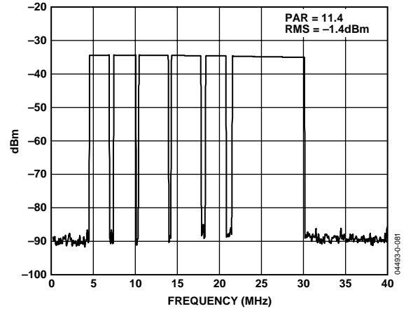
Figure 36. Spectral Plot of 111-Carrier OFDM Test Vector ( f_{DATA} = 80\text{ MSPS} , 2× Interpolation)
