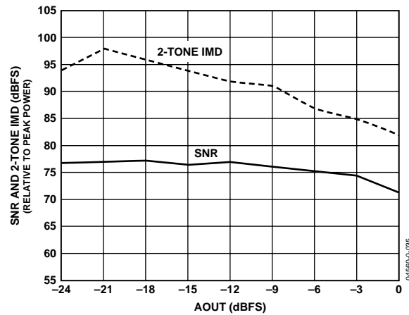
Figure 35. SNR and SFDR vs. P_{OUT} ( f_{OUT} = 12.55\text{ MHz} , f_{DATA} = 50\text{ MSPS} , 4× Interpolation)
