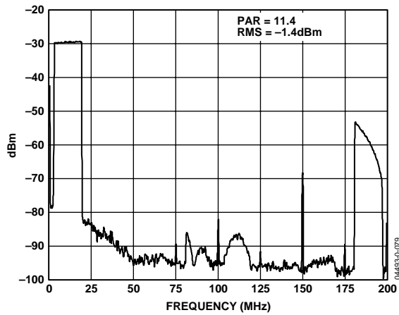
Figure 34. Wideband Spectral Plot of 88-Subcarrier OFDM Test Vector ( f_{DATA} = 50\text{ MSPS} , 4× Interpolation)
