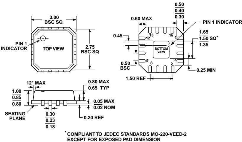
Figure 26. 16-Lead Lead Frame Chip Scale Package [LFCSP] (CP-16) Dimensions shown in millimeters
