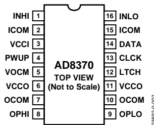
Figure 3.16-Lead TSSOP
