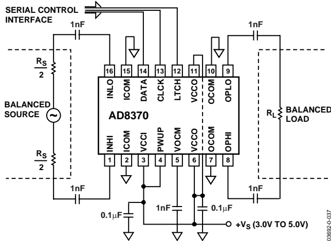
Figure 42. Basic Connections
