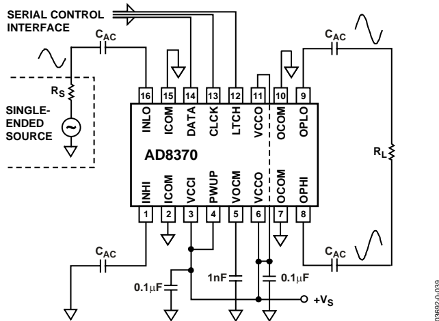
Figure 45. Single-Ended-to-Differential Conversion
