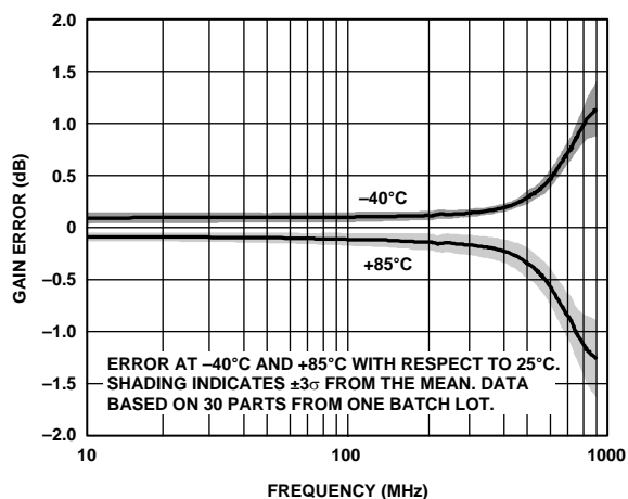
Figure 12. Gain Error over Temperature vs. Frequency, R_L = 100\text{ }\Omega
