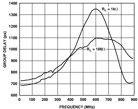
Figure 25. Group Delay vs. Frequency at Maximum Gain
