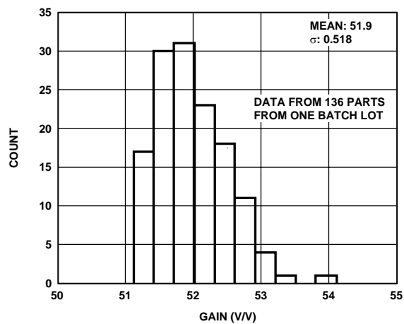
Figure 33. Distribution of Voltage Gain, HG127, 70 MHz, R_L = 100\ \Omega
