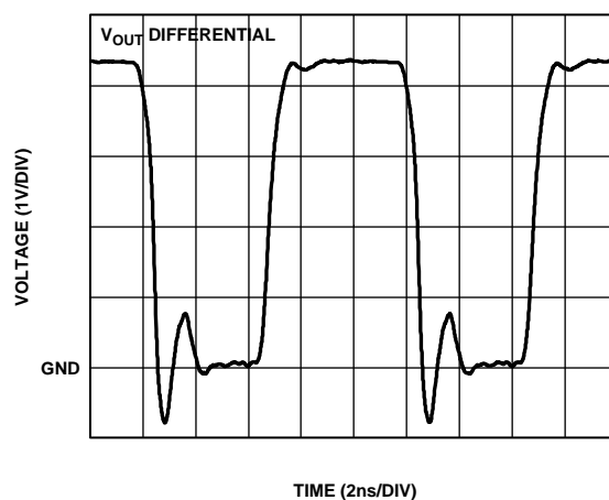
Figure 31. Overdrive Recovery
