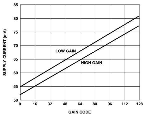
Figure 32. Supply Current vs. Gain Code
