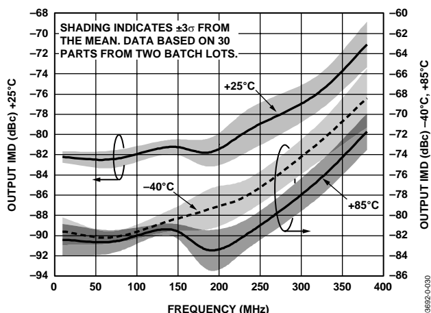
Figure 14. Two-Tone Output IMD3 vs. Frequency at Maximum Gain, R_L = 1\text{ k}\Omega , V_{OUT} = 1\text{ V p-p} Composite Differential
