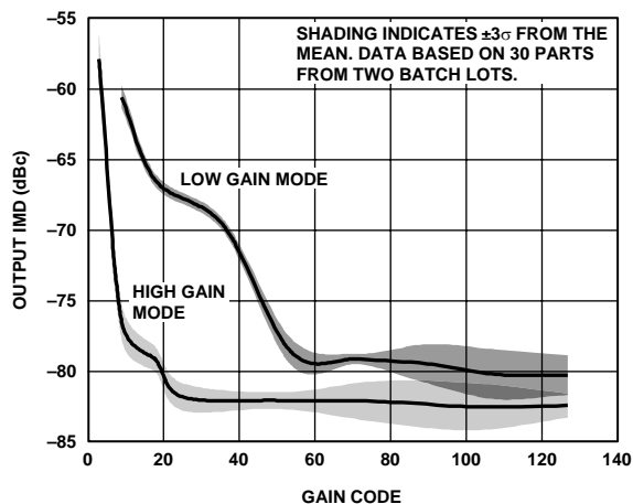
Figure 11. Two-Tone Output IMD3 vs. Gain Code at 70 MHz, R_L = 1\text{ k}\Omega , V_{OUT} = 1\text{ V p-p} Composite Differential
