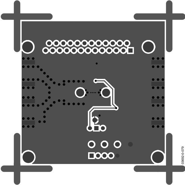
Figure 62. Evaluation Board Bottom
