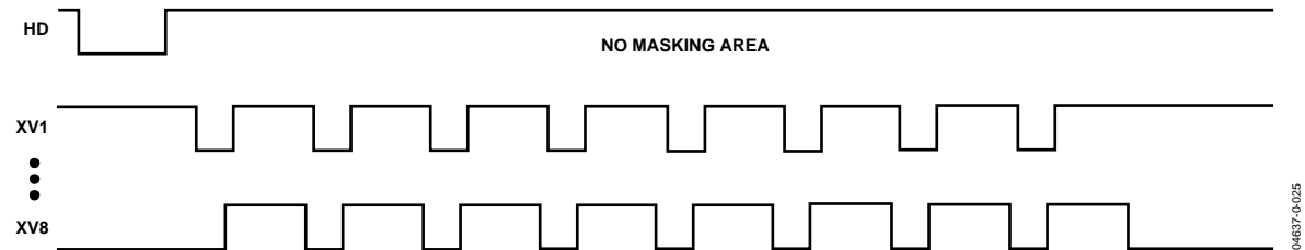
Figure 32. No Vertical Masking
