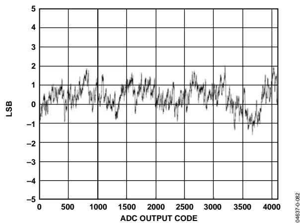
Figure 13. Typical INL Performance
