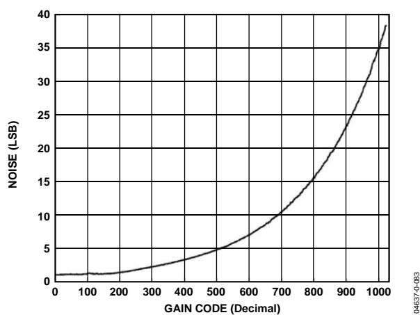
Figure 12. Total Output Noise vs. VGA Gain
