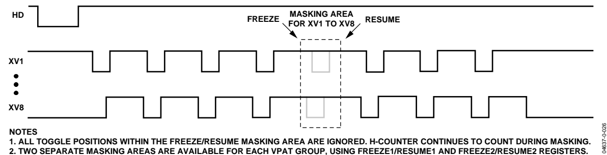
Figure 33. Vertical Masking Using the FREEZE/RESUME Registers
