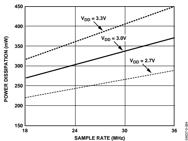
Figure 9. Power vs. Sample Rate
