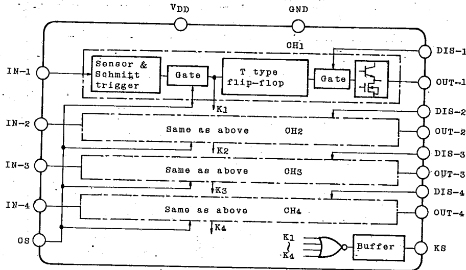
BLOCK DIAGRAM
