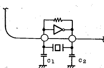
Example using ceramic oscillator Ceramic KBR-455B (Kyoto Ceramics) C 1 , C 2 50 ~ 150pF
