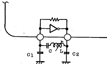
Example using L, C circuit
