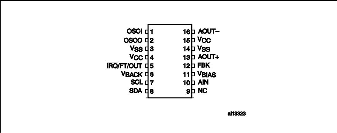
Figure 2. Pin connection
