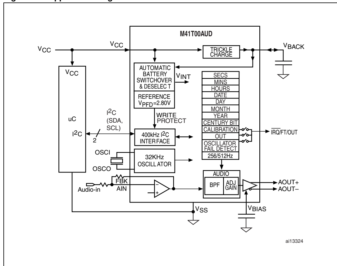
Figure 3. Application diagram
