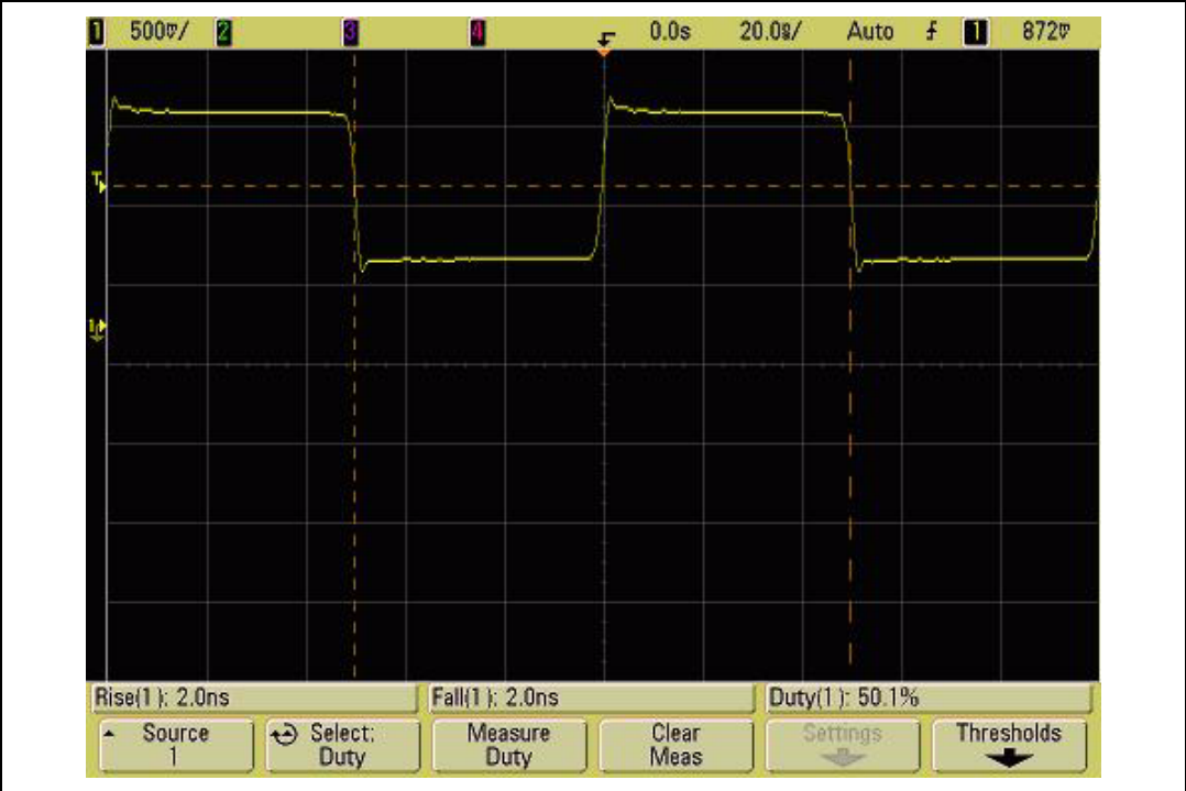
Figure 33. Rise and fall time for square wave output (STCD1040, 1.8 V version, 10MHz square wave master clock input, C load = 20 pF)
