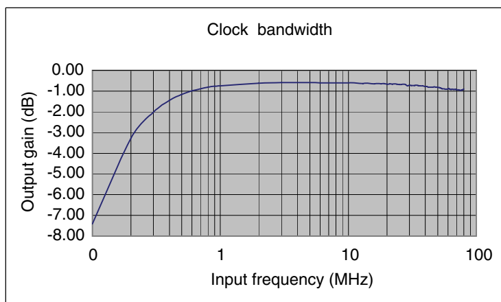
Figure 23. Clock bandwidth (STCD1040, 2.8 V version, C_{load} = 10 pF)
