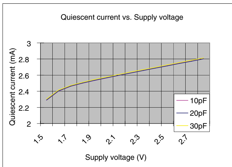
Figure 24. Quiescent current ( I_Q ) vs. supply voltage ( V_{CC} ) (STCD1040, 1.8 V version, EN1=EN2=EN3=EN4=1 , no master clock input)
