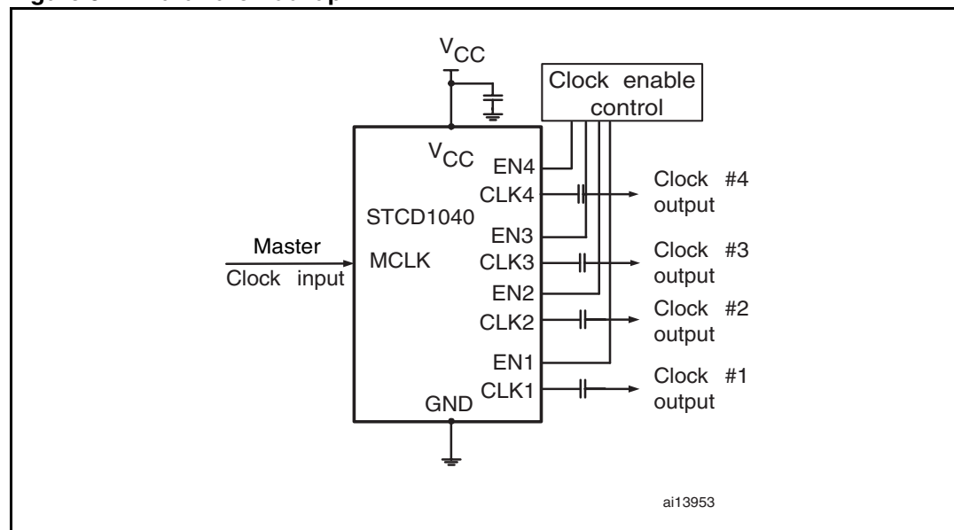
Figure 6. Hardware hookup
