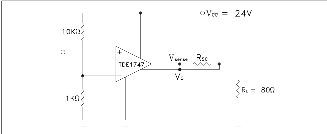
Figure 4. Simplified schematic
