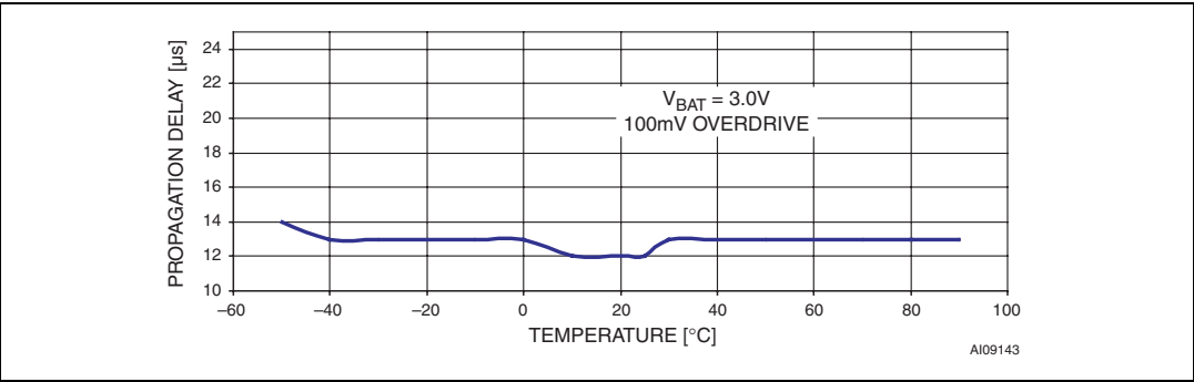
Figure 14. Reset comparator propagation delay vs. temperature
