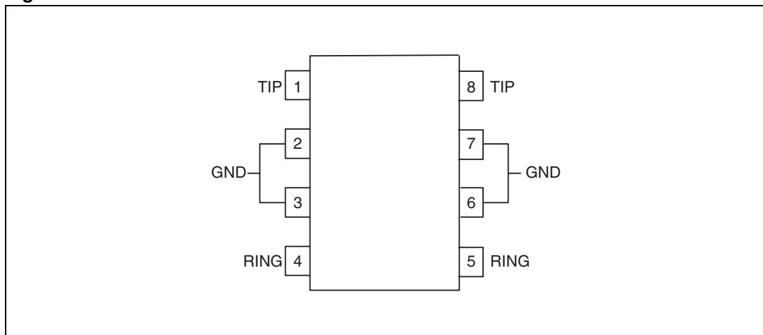
Figure 8. Device connections
