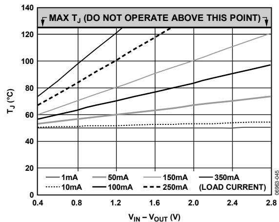
Figure 45. 0 mm² of PCB Copper, T_A = 50^\circ\text{C} , TSOT
