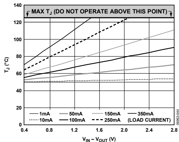
Figure 44. 100 mm² of PCB Copper, T_A = 50^\circ\text{C} , TSOT
