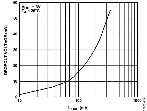
Figure 13. Dropout Voltage vs. Load Current, V_{OUT} = 3\text{ V}
