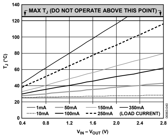
Figure 40. 500 mm² of PCB Copper, T_A = 25^\circ\text{C} , TSOT
