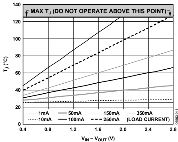
Figure 41. 100 mm² of PCB Copper, T_A = 25^\circ\text{C} , TSOT
