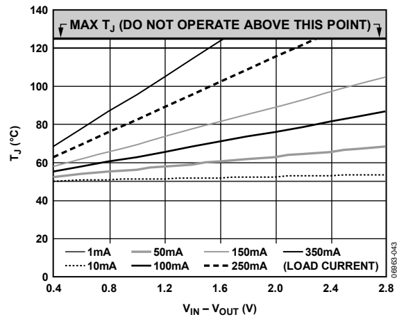
Figure 43. 500 mm² of PCB Copper, T_A = 50^\circ\text{C} , TSOT
