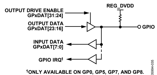
Figure 37. ADuC7036 GPIO
