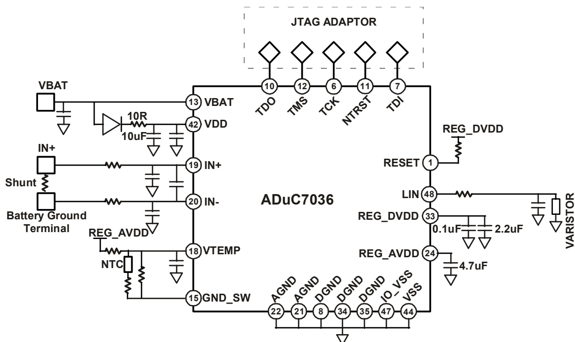
Figure 57. Symplified Schematic
