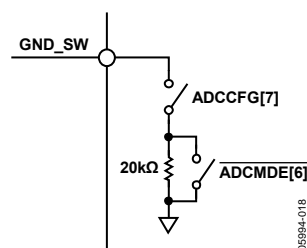
Figure 20. Internal Ground Switch Configuration
