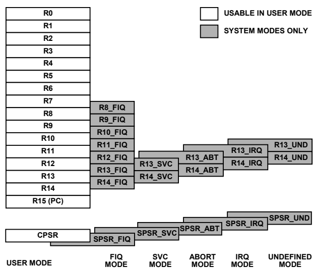
Figure 11. Register Organization
