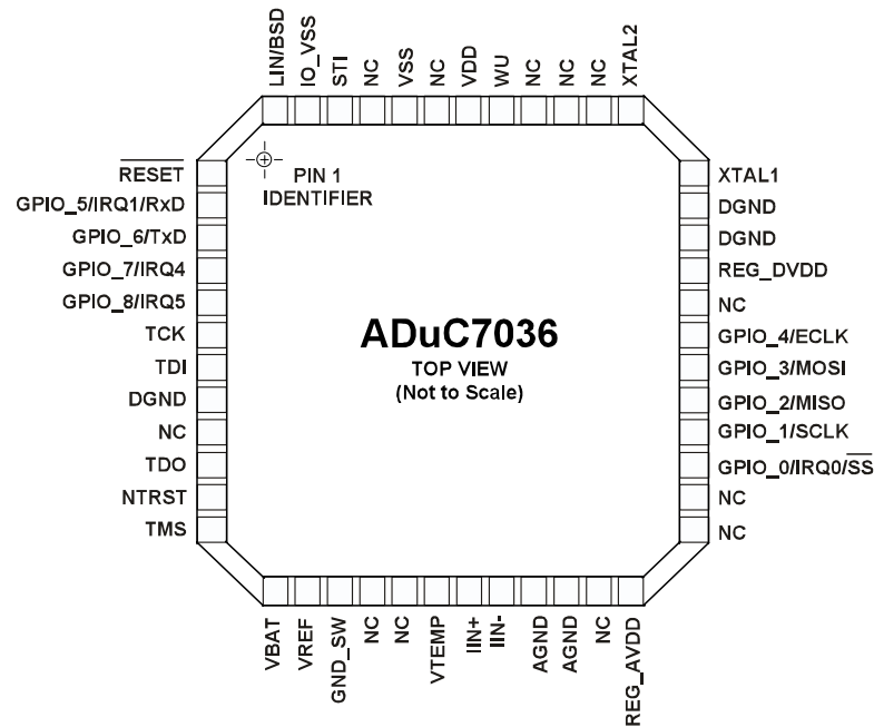
Figure 7. Pin Configuration
