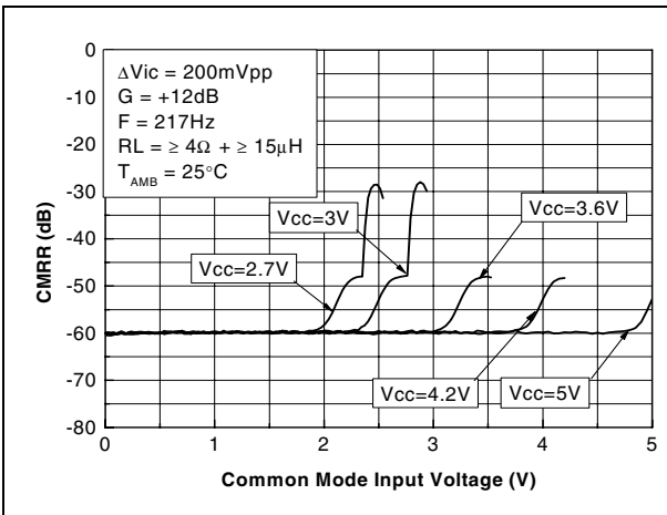
Figure 34. CMRR vs. common mode input voltage
