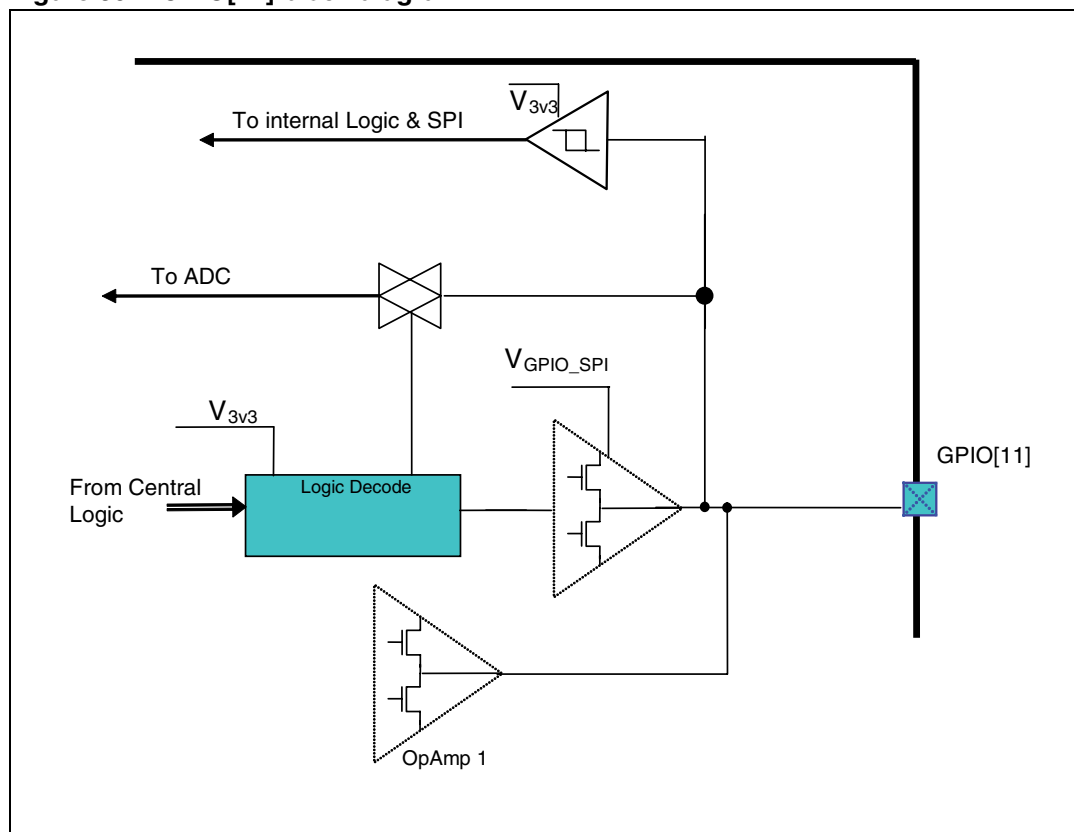
Figure 39. GPIO[11] block diagram
