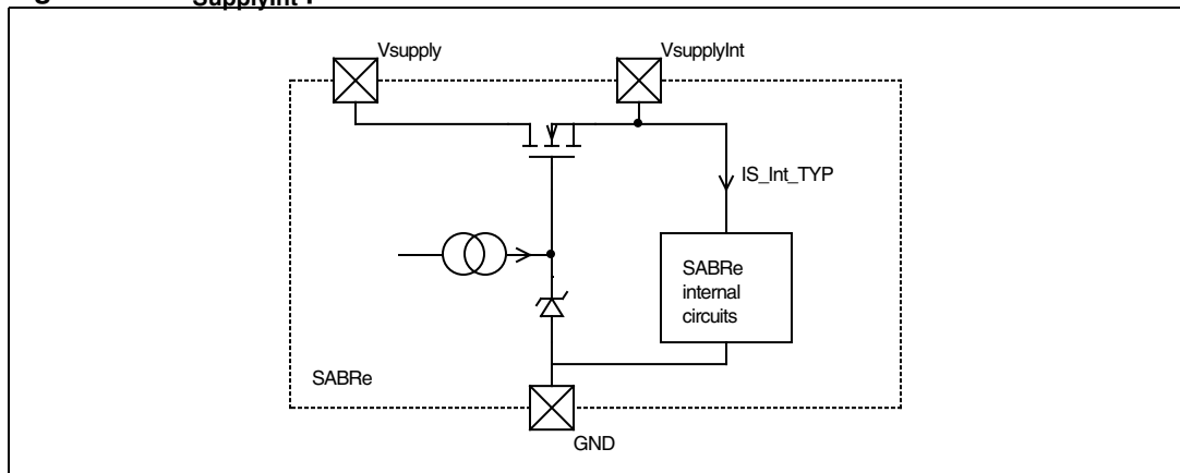
Figure 2. V_{\text{SupplyInt}} pin
