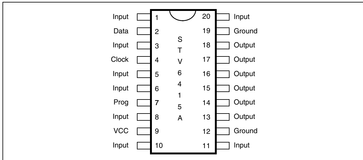
Figure 1. STV6415A Pin-out diagram
