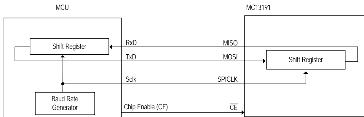
Figure 6. SPI Interface
