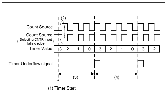
Fig. 62 Timer count start timing and count time when operation starts (Prescaler and Timer 1)
